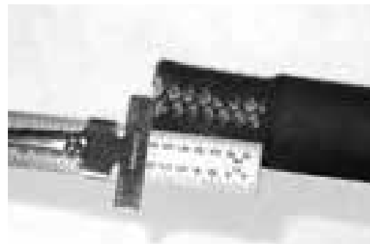
Measure skive.
