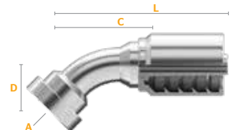
Uni-Crimp™ Style
